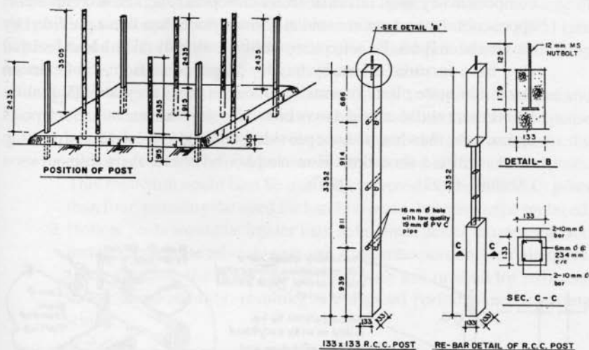
Figure 2 : Typical layout of posts in Grameen Model House
